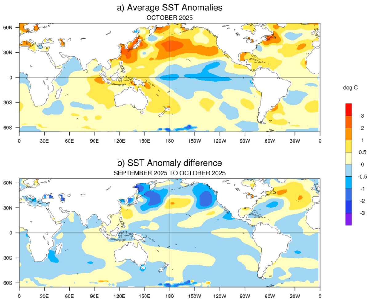
Fig.1: (a) Sea surface temperature (SST) anomalies (degC) during October 2025 and (b) changes in the SST anomalies (degC) from September 2025 to October 2025. SSTs are based on the ERSSTv5 (NCEP-NOAA), and anomalies are computed with respect to 30-year (1991-2020) long term mean.
