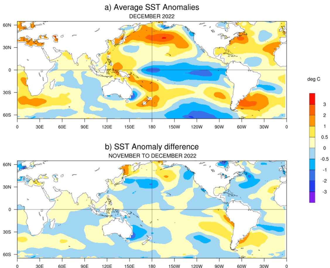
Fig.1: (a) Sea surface temperature (SST) anomalies ( ^{\circ} C) during December 2022 and (b) changes in the SST anomalies ( ^{\circ} C) from November 2022 to December 2022. SSTs were based on the ERSSTv5, NOAA, and anomalies were computed with respect to 30-year (1981-2010) long term mean.
