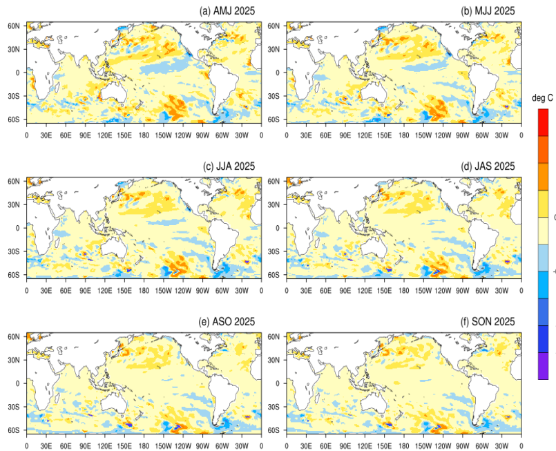
Fig.3: Forecasted Seasonal mean SST anomalies for three-monthly (a) April to June (AMJ 2025), (b) May to July (MJJ 2025), (c) June to August (JJA 2025), (d) July to September (JAS 2025), (e) August to October (ASO 2025) and (f) September to November (SON 2025) (Model bias correction base period: 1999-2008; Climatology base period:1991-2020).
