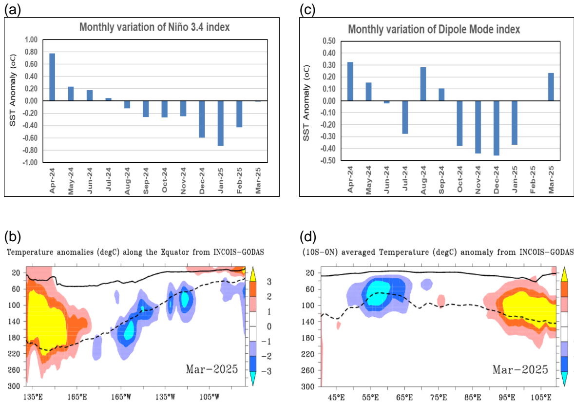
Fig.2: (a) Monthly variation of Niño 3.4 SST index for the last 12 months and (b) Depth-longitude section of sub-surface temperature anomalies in the equatorial (5°S-5°N) Pacific Ocean for the month of March 2025. (c) Same as (a) but for the Dipole Mode Index (DMI). (d) Same as (b) but for the tropical Indian Ocean (10°S-Eq). The anomalies in (a) and (c) were computed using the base period of 1991-2020 (Data Source: ERSSTv5) The solid dark line in (b) and (d) is the 20°C isotherm and the dashed line is thermocline depth (Data Source: INCOIS-GODAS).
