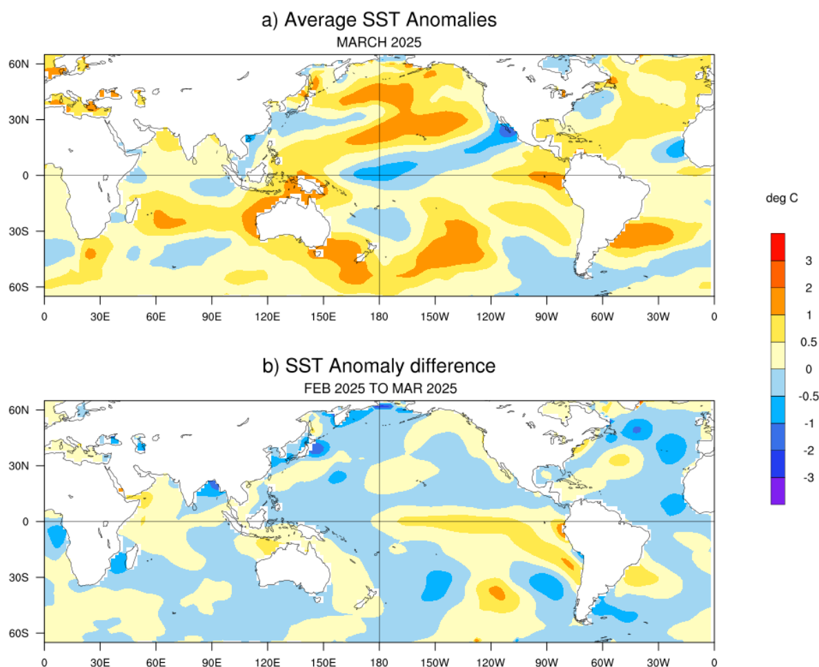
Fig.1: (a) Sea surface temperature (SST) anomalies ( ^{\circ}\text{C} ) during March 2025 and (b) changes in the SST anomalies ( ^{\circ}\text{C} ) from February 2025 to March 2025. SSTs are based on the ERSSTv5 (NCEP-NOAA), and anomalies are computed with respect to 30-year (1991-2020) long term mean.
