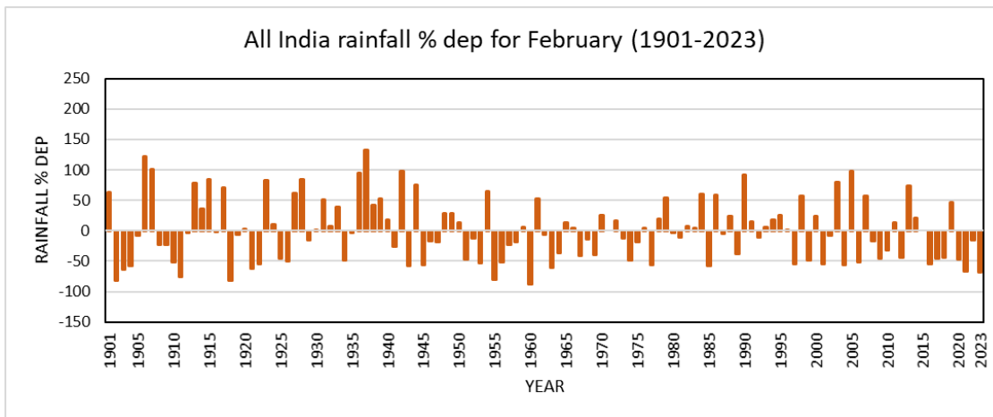
Fig 1(b). All India monthly rainfall percentage departure from normal (1971-2020) for February from 1901-2023.
