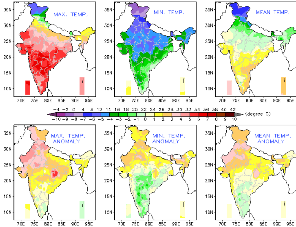
Fig 10: Observed spatial temperature pattern of monthly average maximum, average minimum and mean temperature over India (top three from left to right) and their departure from normal (1981 to 2010 period) for February 2023 (lower three from left to right).
