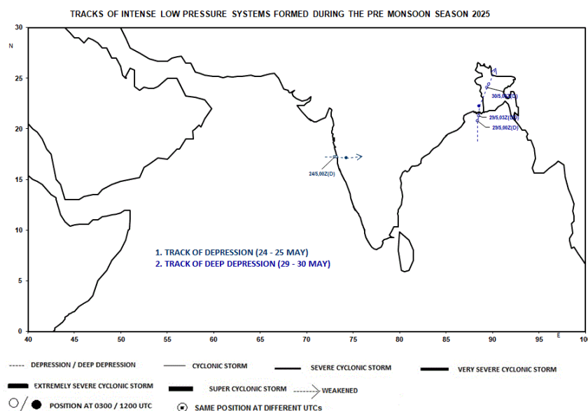
Fig 7: Tracks of low pressure systems during May 2025.
