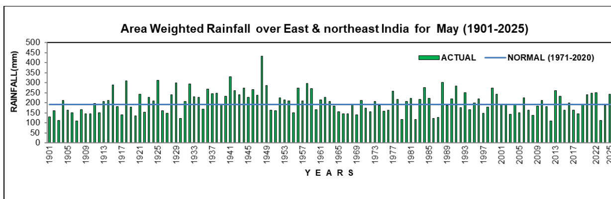
Fig 1(g). Time series of area weighted rainfall over East & northeast India for May (1901 – 2025).
