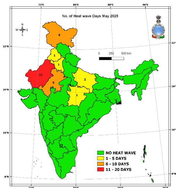
Fig 8: Subdivision-wise heat wave days during May 2025.
