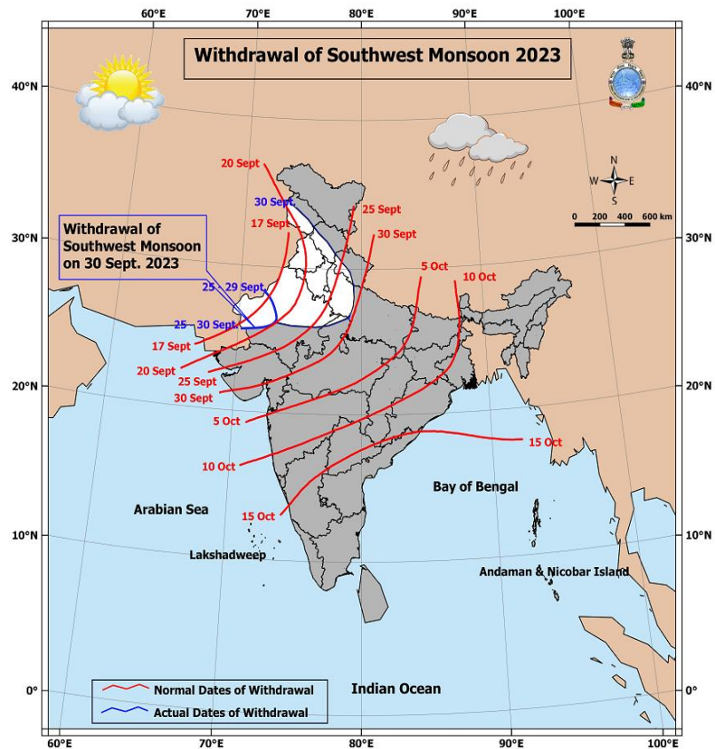
Fig.2: Isochrones of withdrawal of southwest monsoon – 2023 as on 30 Sep. 2023.
