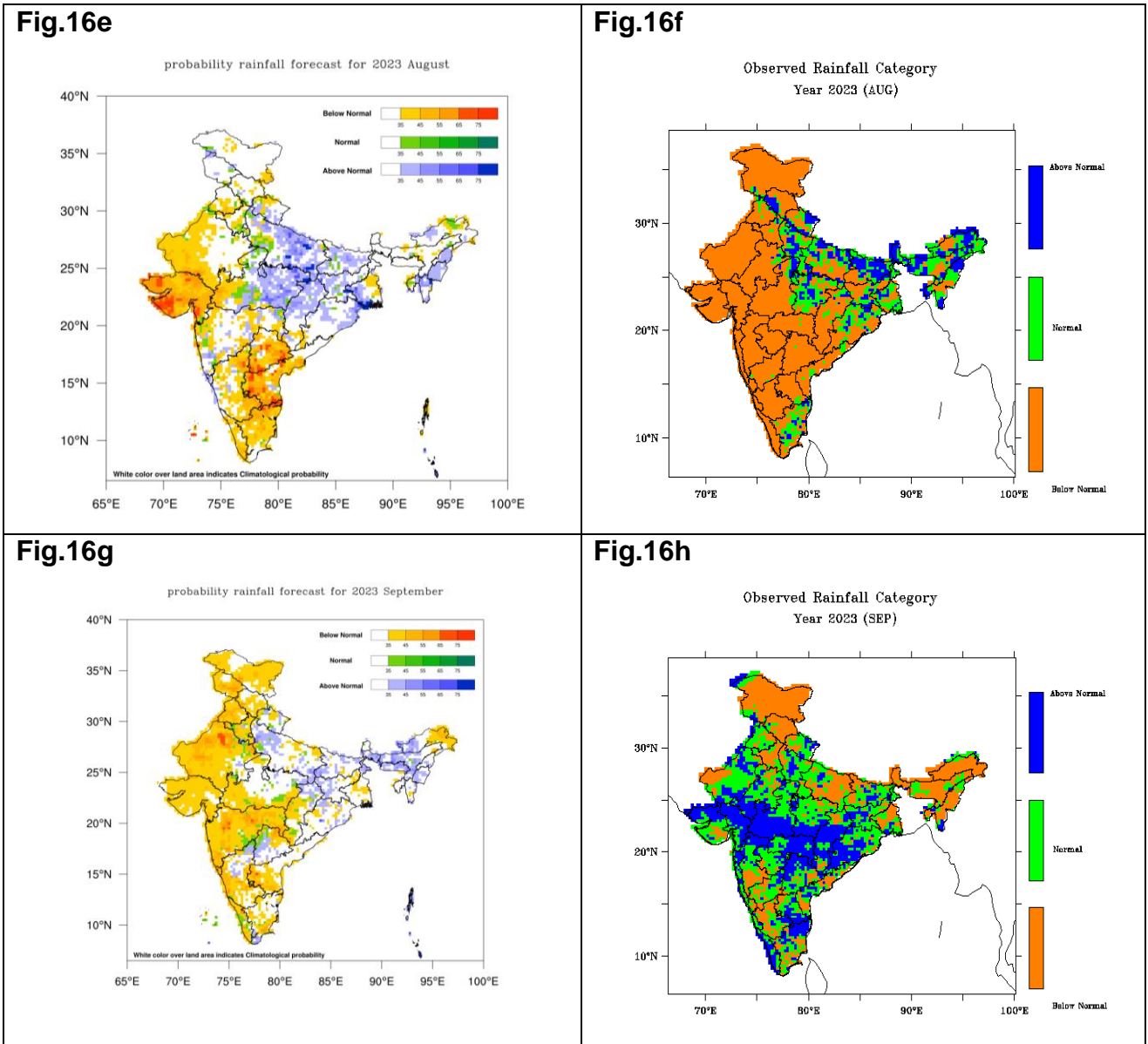
Fig.16. Verification of the spatial forecast for monthly rainfall from June to September 2023, with corresponding observed rainfall categories provided in (a and b) for June, (c and d) for July, (e and f) for August and (g and h) for September 2023.
