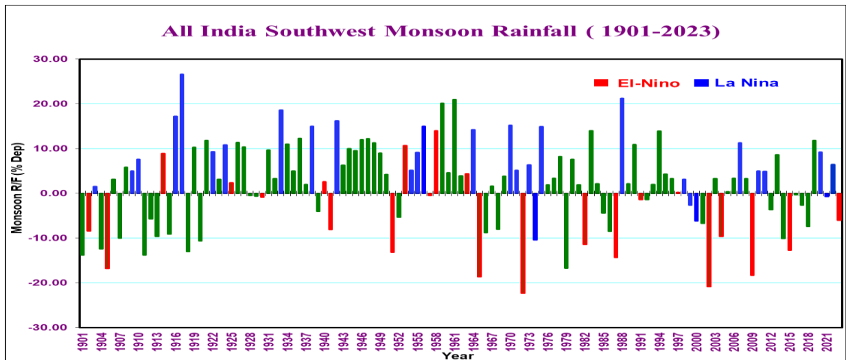
Fig.11: Inter-annual variability of All India Summer Monsoon Rainfall
