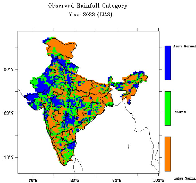
Fig.15. (a and b). Spatial forecast for the seasonal rainfall from June to September 2023, corresponding to the first stage (issued in April) and second stage (issued in May), respectively, (c) observed rainfall category.
