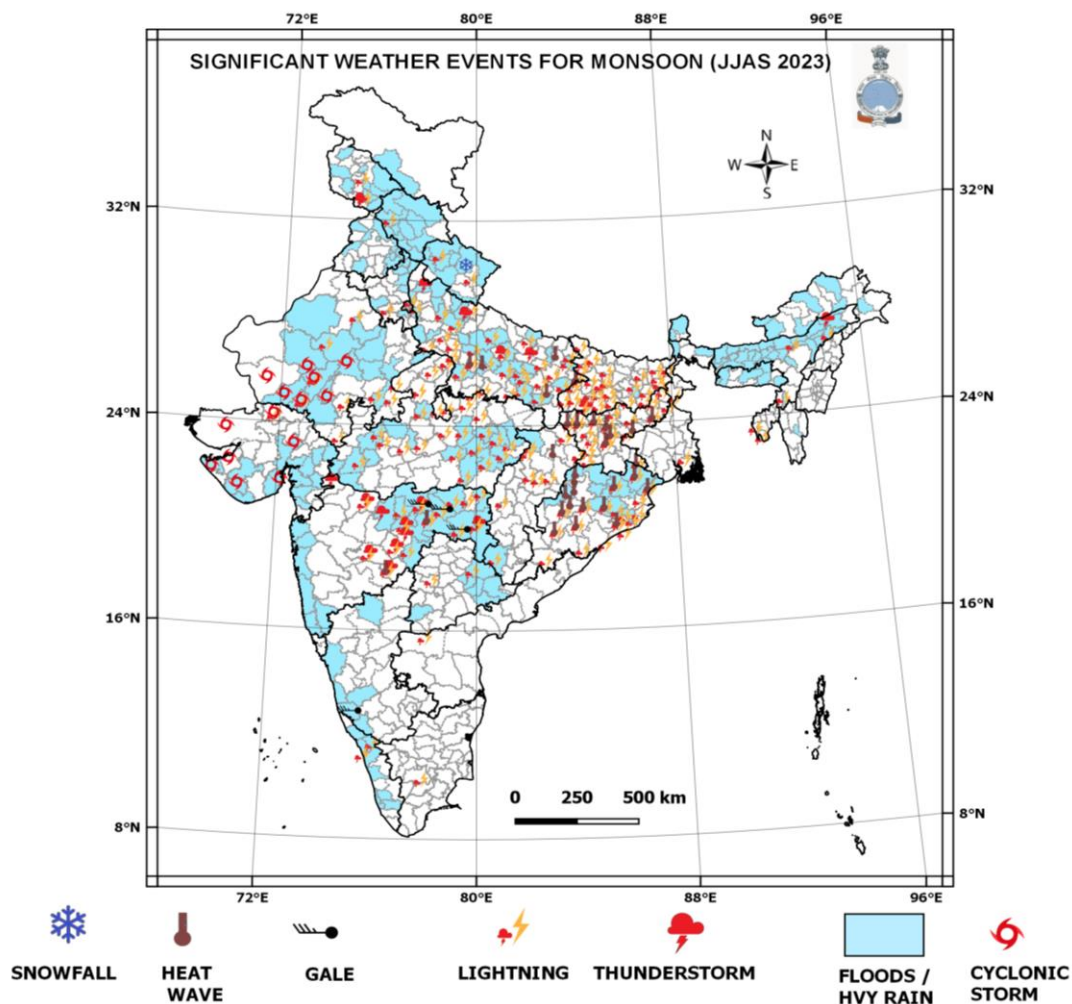
Fig.10: Significant weather events in the southwest monsoon 2023 season causing disastrous situations.
