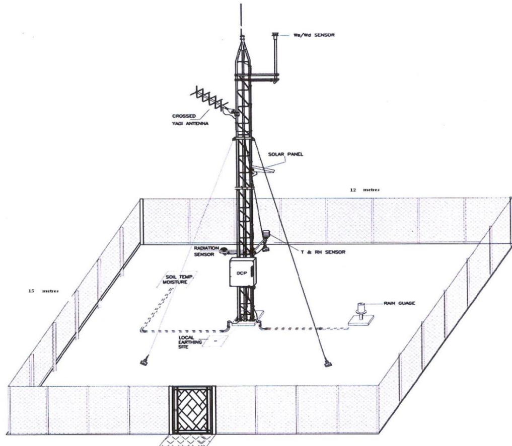
SCHEMATIC VIEW OF AWS SITE
